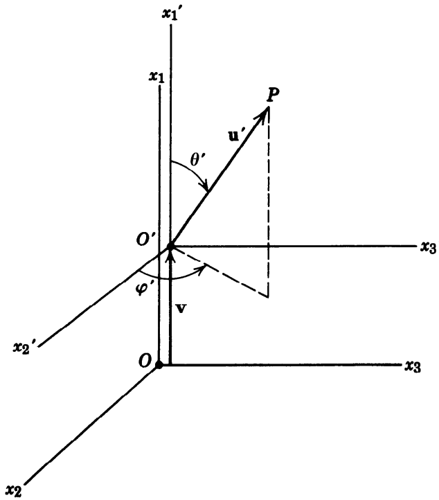
Figure 11.4 Addition of velocities.
