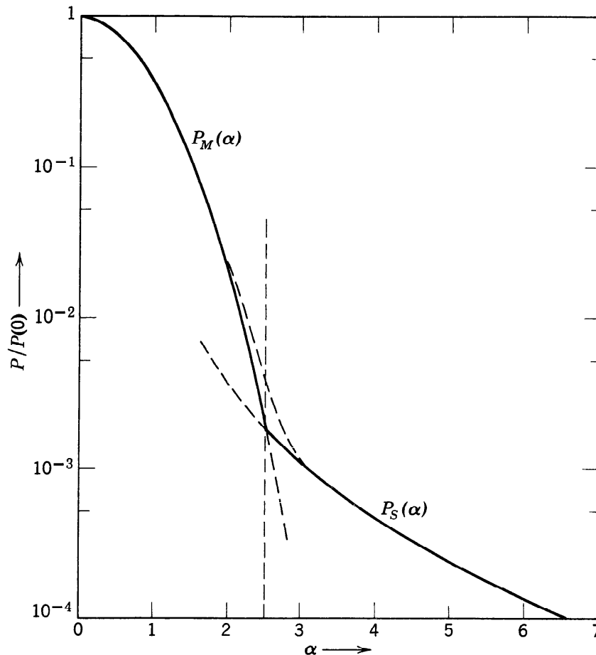
Figure 13.8 Multiple- and single-scattering distributions of projected angle. In the region of plural scattering ( \alpha \sim 2\text{--}3 ) the dashed curve indicates the smooth transition from the small-angle multiple scattering (approximately Gaussian in shape) to the wide-angle single scattering (proportional to \alpha^{-3} ).
