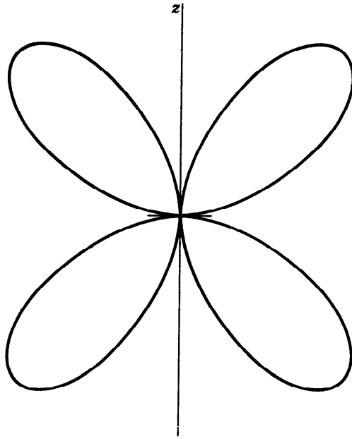
Figure 9.2 A quadrupole radiation pattern.
