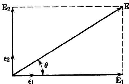
Figure 7.2 Electric field of a linearly polarized wave.
