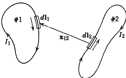
Figure 5.3 Two Ampèrian current loops.
