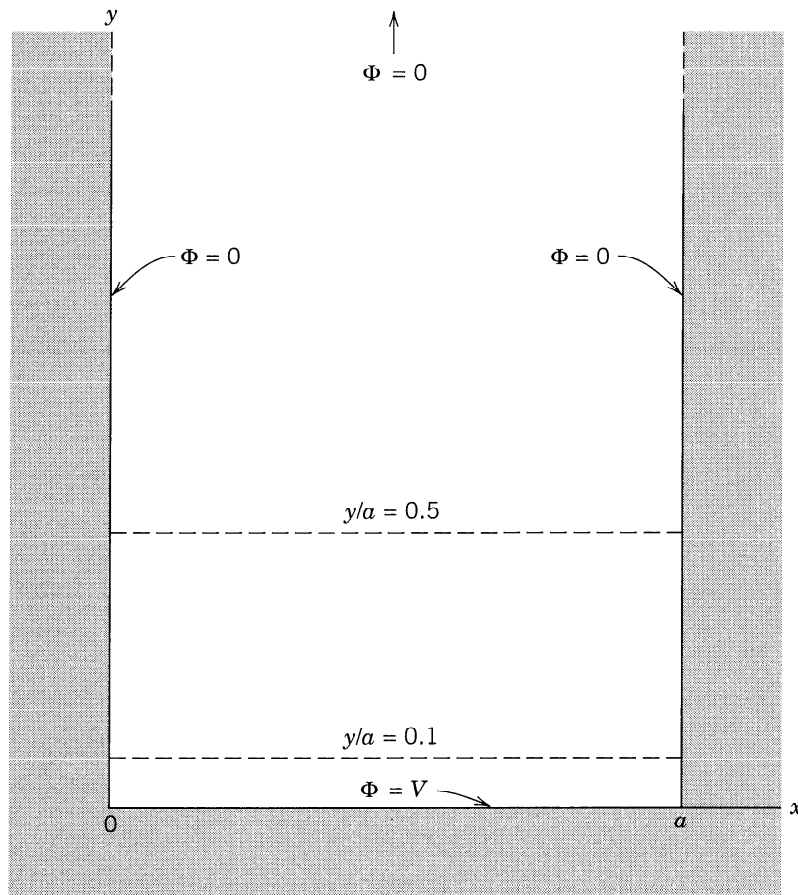
Figure 2.10 Two-dimensional potential problem.
