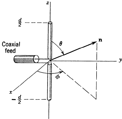
Figure 9.3 Center-fed, linear antenna.
