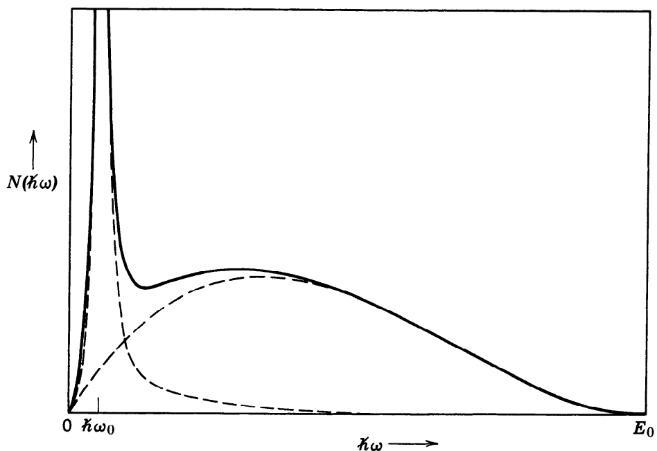
Figure 15.13 Typical photon spectrum for radiative orbital-electron capture with energy release E_0 , showing the contributions from the disappearance of the electronic charge and magnetic moment.
