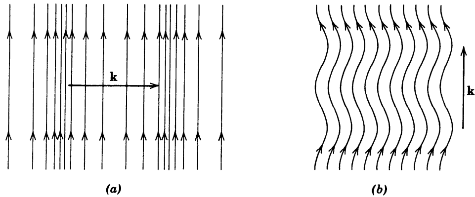
Figure 7.12 Magnetohydrodynamic waves.
