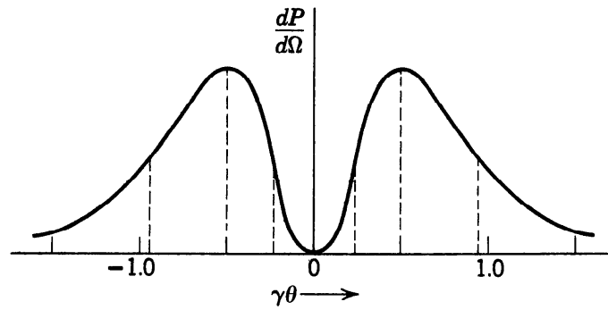
Figure 14.5 Angular distribution of radiation for relativistic particle.
