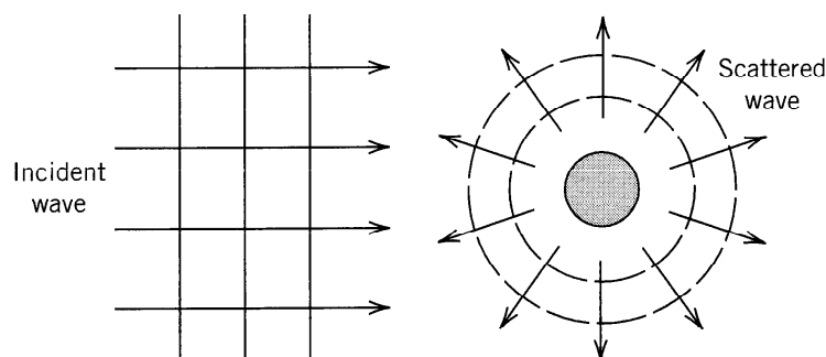
Figure 10.6 Scattering of radiation by a localized object.
