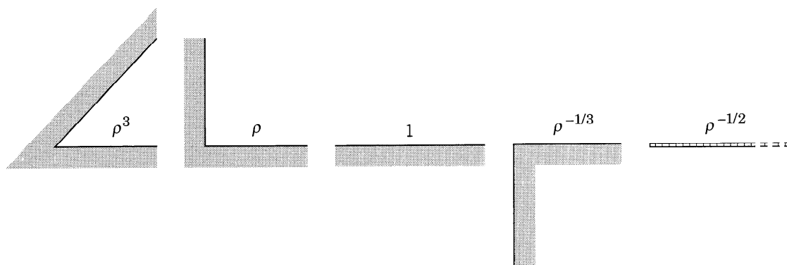
Figure 2.13 Variation of the surface-charge density (and the electric field) with distance \rho from the “corner” or edge for opening angles \beta = \pi/4, \pi/2, \pi, 3\pi/2, \text{ and } 2\pi .
