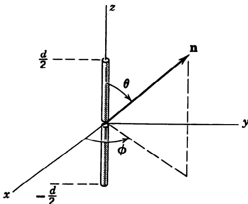
Figure 9.1 Short, center-fed, linear antenna.
