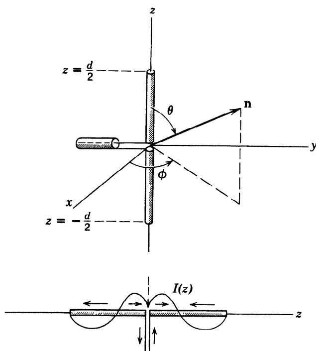
Figure 9.6 Linear, center-fed antenna.
