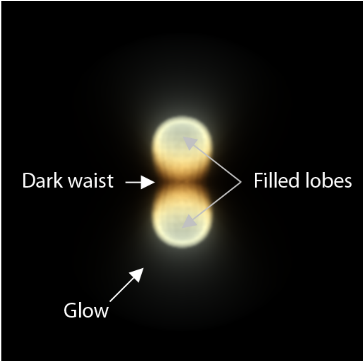
Fig. 2.— Rendered image of the model. Several features commonly seen in reflection nebulae are evident in this simple model, including a dark waist and the appearance of volume filled lobes.
