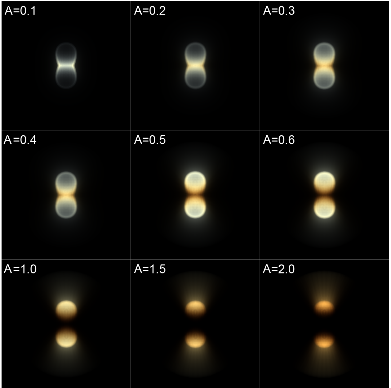
Fig. 3.— Simulation results for different densities in the dust halo. The images are displayed on a linear intensity scale. The density parameter A is marked on each frame. As the density increases, the dust lane thickens, the searchlight beams become more prominent and the shell morphology gives way to a more volume filled appearance.
