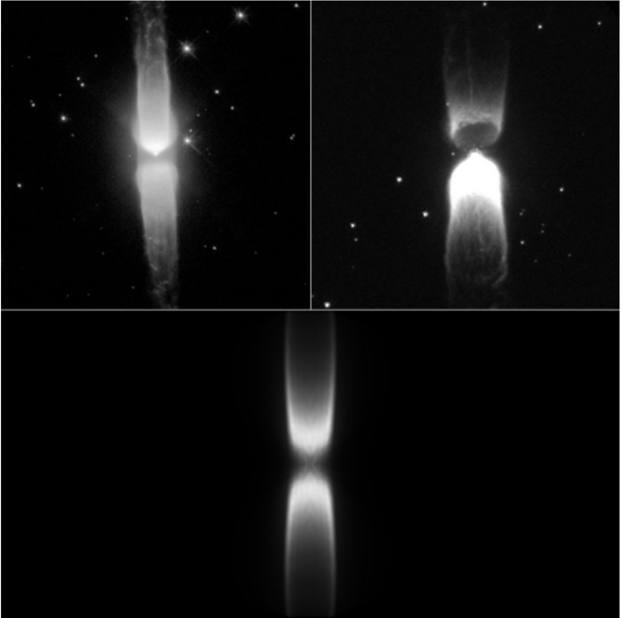
Fig. 5.— Comparisons between observed reflection nebulae with cylindrical shapes to the model. As the size of the bipolar cavity increases, the curved nature of the lobes disappears and a more cylindrical morphology emerges. Top left: IRAS 10178–5958 (Hen 3-401) (image created from the NASA/ESA/STScI, Hubble Archives, Project GO6816, PI: Sahai). Top right: IRAS 13208-6020 (Image created from NASA/ESA/STScI, Hubble Archives, Project GO10546, PI: Sahai). Bottom: Model image with a cavity \ell factor of 5.
