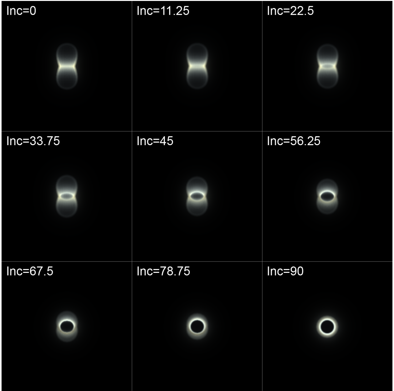
Fig. 7.— Simulated images as viewed from different directions for the low-density ( A=0.1 \text{ m}^{-1} ) case. The inclination angle of each simulation is indicated in the image panels. As the inclination increases, a ring like structure appears in the center surrounded by a faint elliptical structure.
