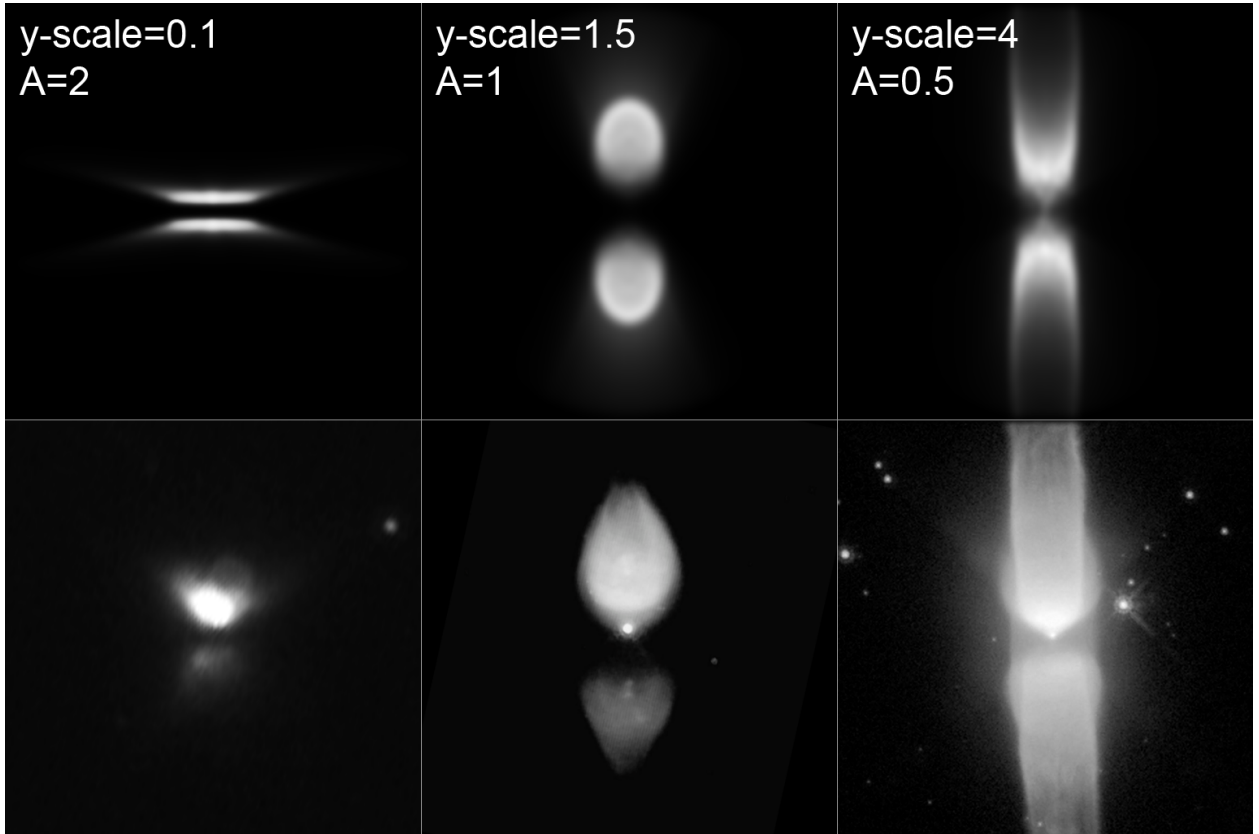
Fig. 12.— Top row: a simulation of evolutionary progression in morphology as the lobes get larger and the density of the dust halo drops. Evolution in age is from left to right. The model parameters are given in each of the three panels. A Gaussian convolution was applied to simulate the diffraction pattern of the telescope. Bottom row: observed images selected as examples of possible observational counterparts of the simulated images. From left to right: IRAS 13557-6442 (image created from NASA/ESA/STScI, Hubble Archives, Project GO9463, PI Sahai); IRAS 19343+2926 (image created from NASA/ESA/STScI, Hubble Archives, Project GO6533, PI Buharrabal); IRAS 10178–5958 (image created from NASA/ESA/STScI, Hubble Archives, Project GO6816, PI Sahai).
