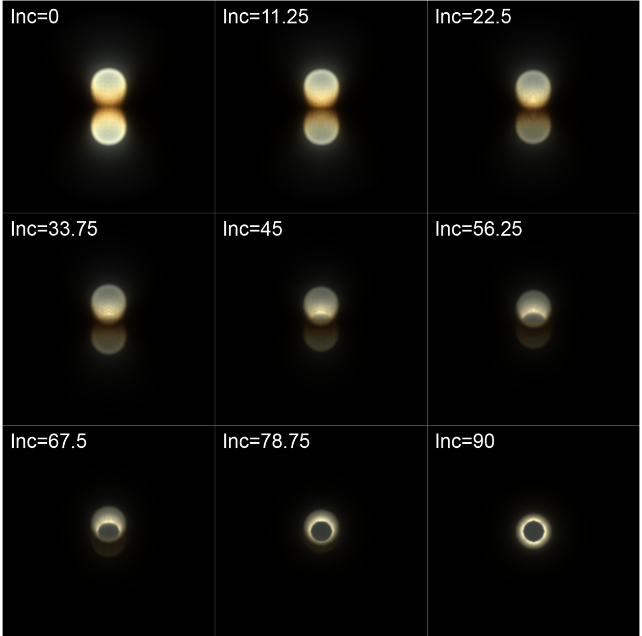
Fig. 6.— Simulated images as viewed from different directions. The inclination angle is marked on each frame. The model is for the case A=0.5 \text{ m}^{-1} . As the inclination increases, the back lobe becomes fainter and the dust lane takes on a torus appearance.
