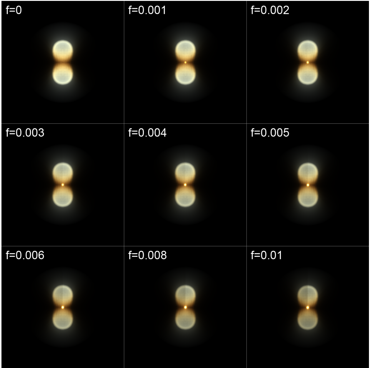
Fig. 10.— Simulated images showing the effect of having small traces of dust remaining in the cavity. The cavity density is given by n_c(r) = fn_0(r) , where n_0(r) is the dust density in the envelope at distance r from the central star. The brightness scale for all images has been normalized to the first image at f = 0 .
