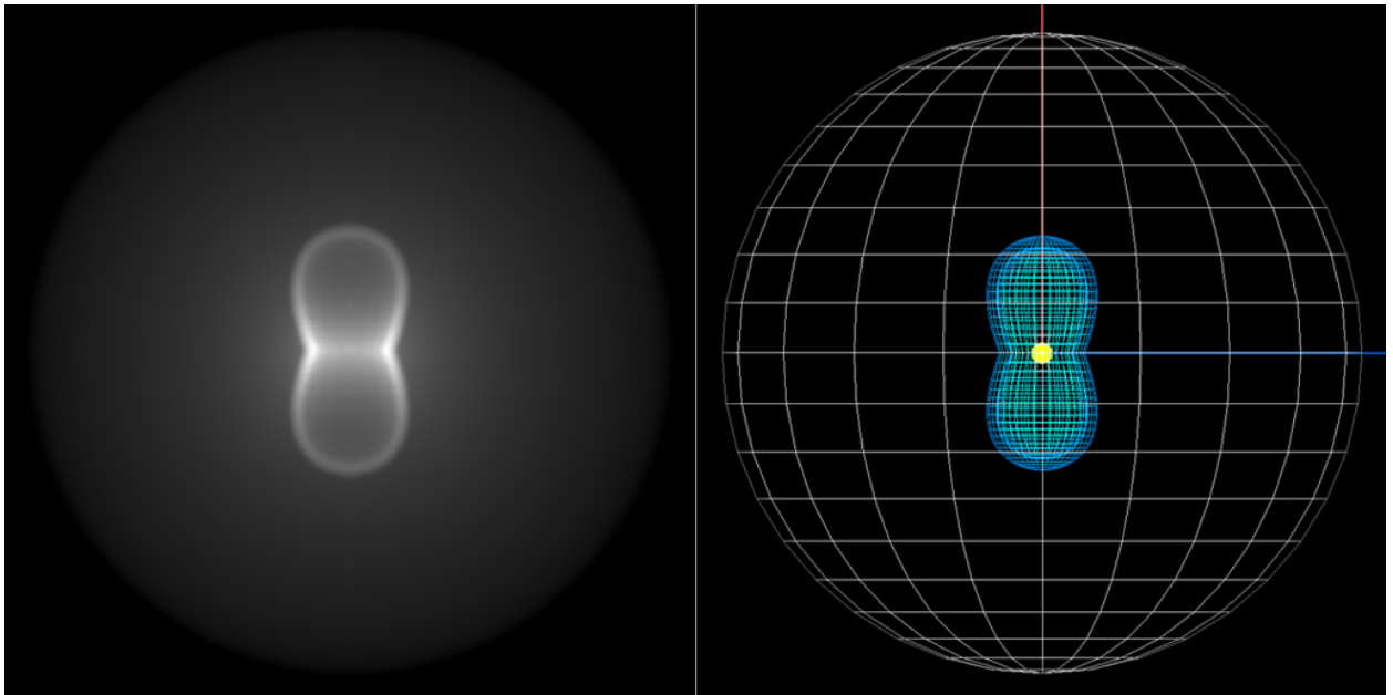
Fig. 1.— Left: a grey scale presentation of the column density distribution of the model from a view perpendicular to the bipolar axis. The brightness of the image is presented on a square-root scale. Right: a mesh presentation of the model.
