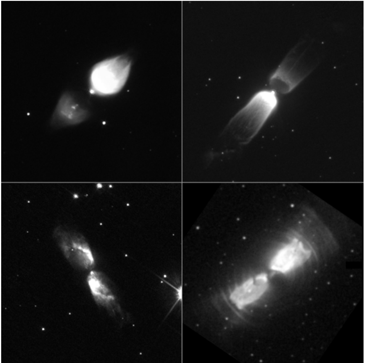
Fig. 11.— Example of several bipolar reflection nebulae and proto-planetary nebulae that display a bright central “star-like” region. From left to right, top to bottom: M1-92 (image created from NASA/ESA/STScI, Hubble Archives, Project GO6533, PI Buharrabal); IRAS 13208-6020 (image created from NASA/ESA/STScI, Hubble Archives, Project GO10536, PI Sahai); IRAS 20068+4051 (image created from NASA/ESA/STScI, Hubble Archives, Project GO10536, PI Sahai), IRAS 17150-3224 (image created from NASA/ESA/STScI, Hubble Archives, Project GO6565, PI Kwok).
