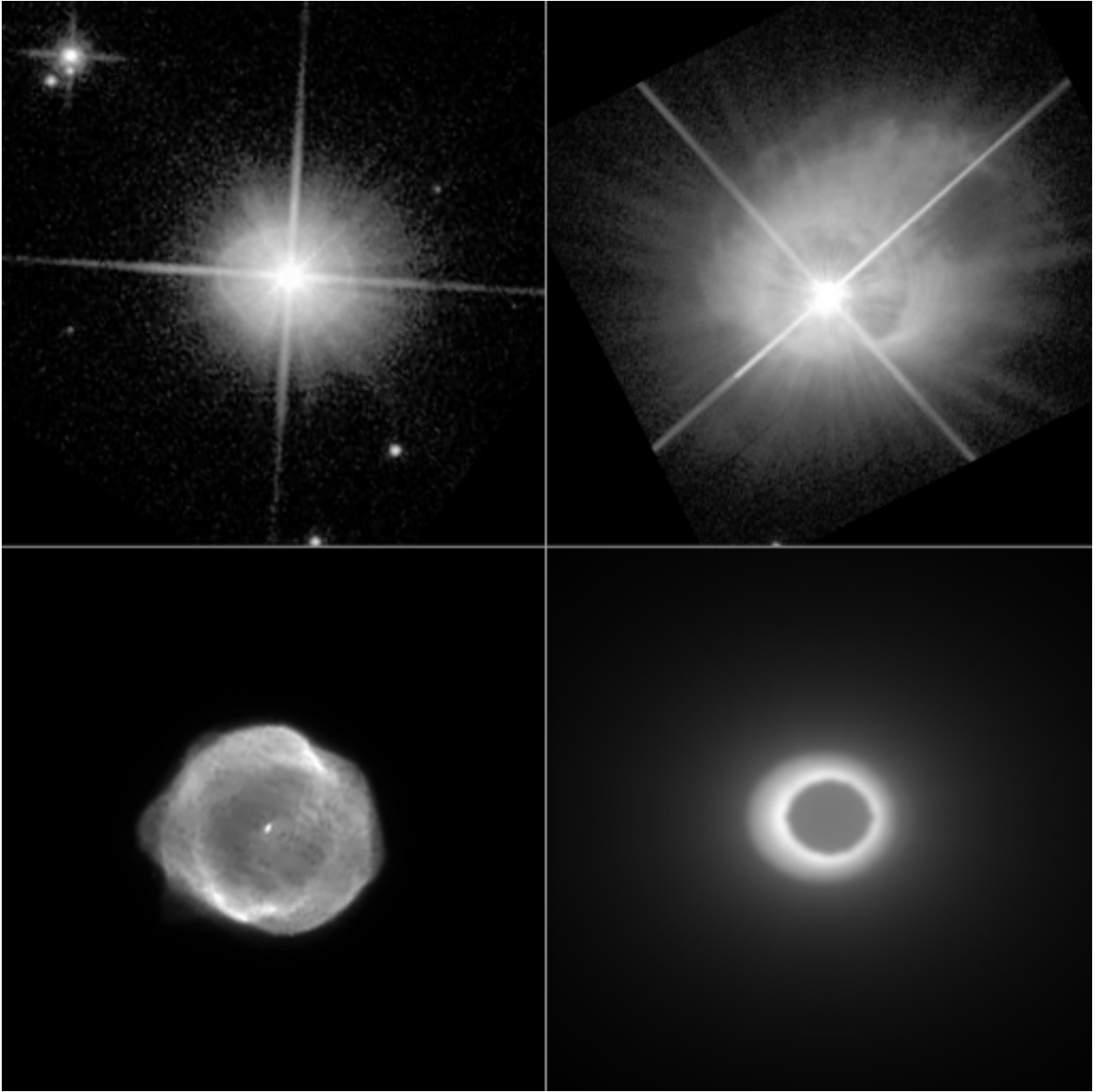
Fig. 9.— When viewed pole on, the model (bottom right) appears ring-like surrounded by a faint outer halo. This morphology is similar to some PPNs (top images) and many young PNs (bottom left image). Left to right, top to bottom: IRAS 20462+3416 (image created from NASA/ESA/STScI, Hubble Archives, Project GO6364, PI Bobrowsky); IRAS 11385–5517 (image created from NASA/ESA/STScI, Hubble Archives, Project GO69463, PI: Sahai); IRAS 15318-7144 (Young PN) (image created from NASA/ESA/STScI, Hubble Archives, Project GO6119/6353, PI Bond/Sahai); model image at an inclination of 90^\circ and A=0.5 \text{ m}^{-1} . Direct light from the central star is not rendered in the model image.
