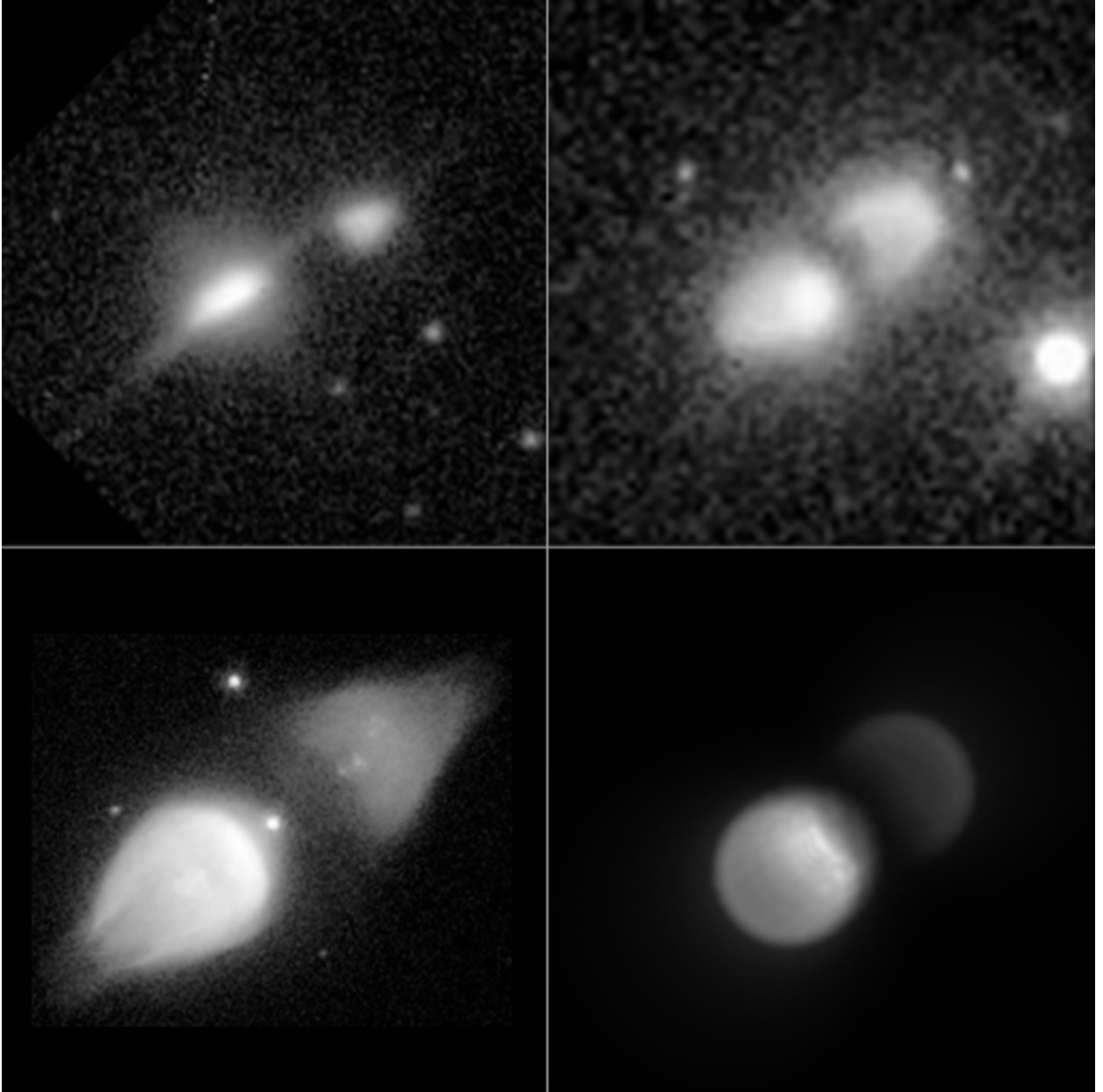
Fig. 8.— Many bipolar reflection nebulae show a well-defined, thick “torus” around their waist. This morphology is well reproduced by the model at a non-zero inclination angle. . From left to right, top to bottom: IRAS 16243-3814 (image created from NASA/ESA/STScI, Hubble Archives, Project GO6364, PI Bobrowsky); IRAS 19292+1806 (image created from NASA/ESA/STScI, Hubble Archives, Project GO9463, PI Sahai); IRAS 19343+2926 (image created from NASA/ESA/STScI, Hubble Archives, Project GO6533, PI Buharrabal); model image for the density parameter A=0.5 \text{ m}^{-1} with an inclination of 45^\circ .
