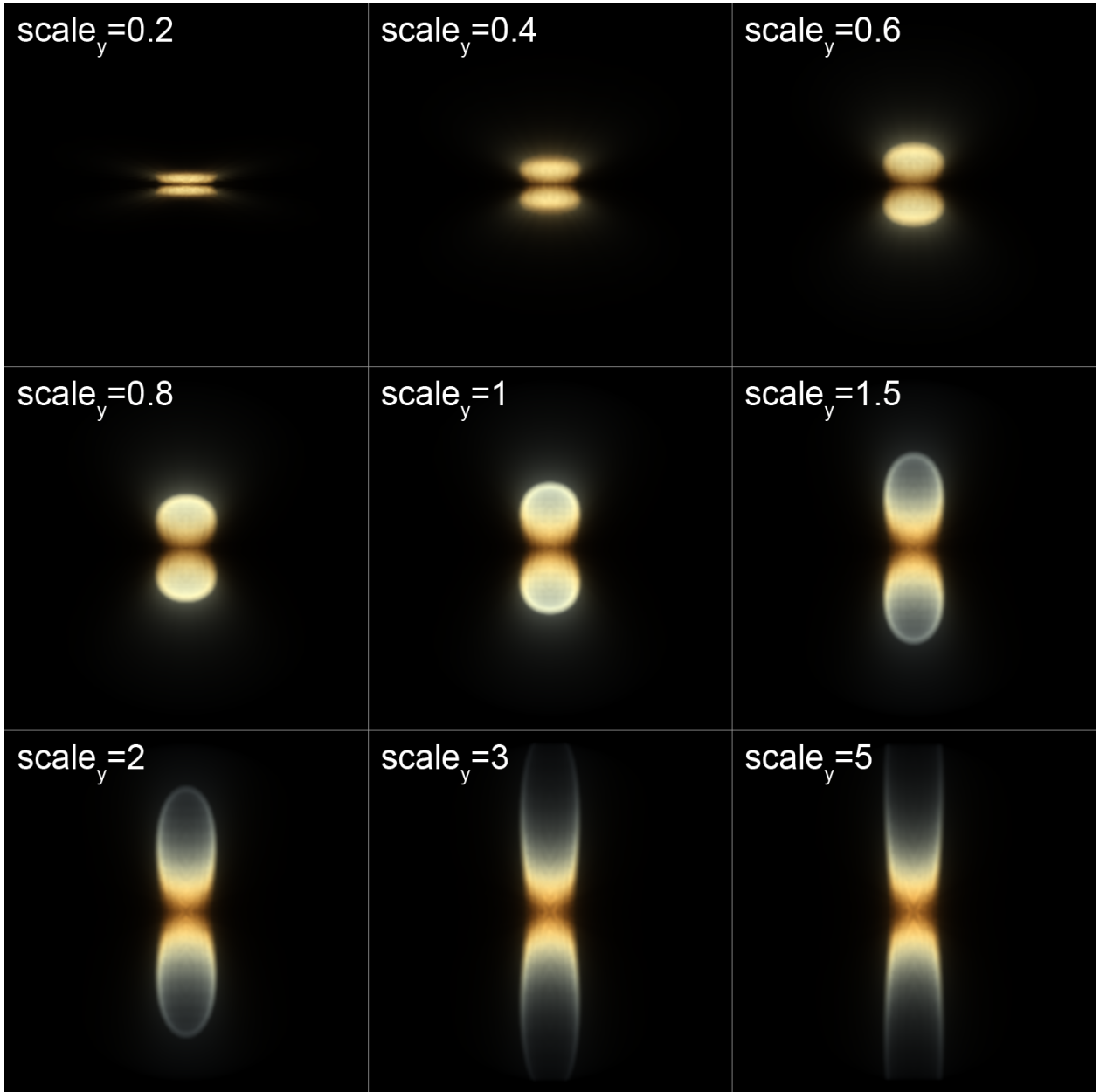
Fig. 4.— Simulated images as the result of varying sizes of the cavity in one ( y ) direction. The size scale ( \ell ) ranges from 0.2 to 5. A scale of 1 corresponds to a lobe size of 1'' . As the scale increases, the cavity displays a more shell-like morphology and the curved bipolar lobes give way to a more cylindrical look.
